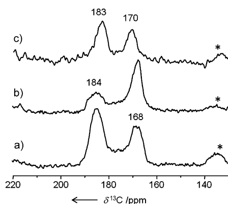
Figure 3. ^{13}\text{C} CP-MAS NMR spectra of ^{13}\text{CH}_3^{13}\text{COCl} adsorbed on H-Beta zeolite at room temperature and a) heated at 333 K for 2 h, before being b) outgassed at 333 K for 1 h. c) The reaction mixture ^{13}\text{CO}/^{13}\text{CH}_3\text{OH} (molar ratio = 3:1) on H-Mordenite zeolite heated at 473 K for 1 min. Asterisks denote spinning side bands.
