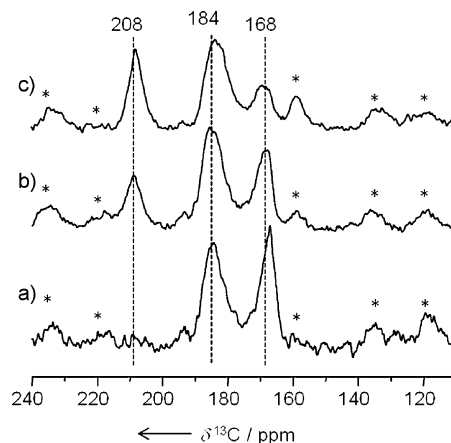
Figure 2. ^{13}\text{C} MAS NMR spectra of the ^{13}\text{CH}_3^{13}\text{COCl} /anisole (molar ratio = 1:1) reaction mixture a) adsorbed at room temperature on H-Beta zeolite. The same sample was then heated at 363 K for b) 90 min and c) 300 min. Asterisks denote spinning side bands.
