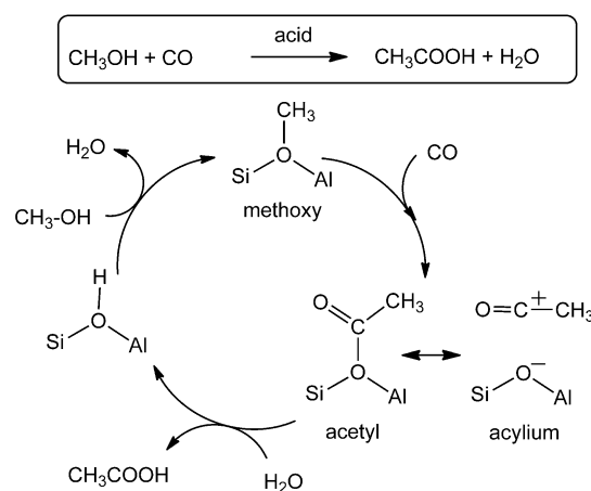
Scheme 2. Carbonylation of methanol with CO over acid zeolites.
