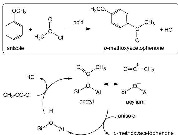
Scheme 1. Friedel–Crafts acylation of anisole over acid zeolites.
