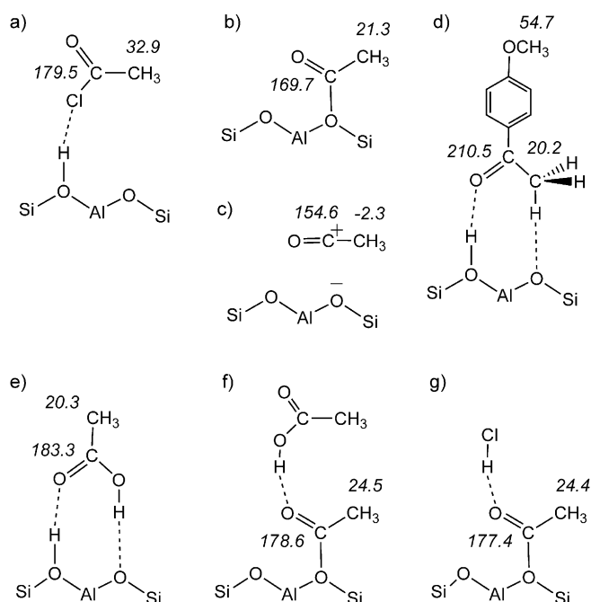
Figure 1. Calculated ^{13}\text{C} isotropic chemical shifts of a) acetyl chloride adsorbed on a Brønsted acid site, b) acetyl group covalently bound to a zeolite framework oxygen, c) cationic acylium–zeolite complex, d) para -methoxy acetophenone adsorbed on a Brønsted acid site, e) acetic acid adsorbed on a Brønsted acid site, f) covalently bound acetyl interacting with acetic acid, and g) covalently bound acetyl interacting with HCl. The numbers in italics are the calculated isotropic ^{13}\text{C} NMR chemical shifts of the associated carbon atoms.
